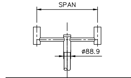
TWIN "COWHORN" POST TOP BRACKET
