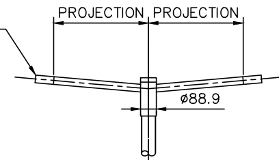
TWIN DROP-OVER BRACKET
