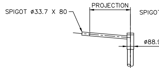
SINGLE DROP-OVER BRACKET
