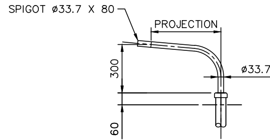
SINGLE ARM BRACKET "METRO 47" & "METRO 57" ONLY
