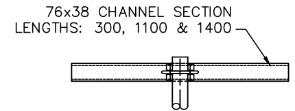
FLOODLIGHT CROSSARM BRACKET
