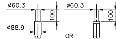
60.3 POST TOP SPIGOT ADAPTORS
