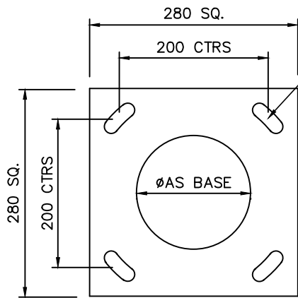
FLANGE PLATE DETAIL
