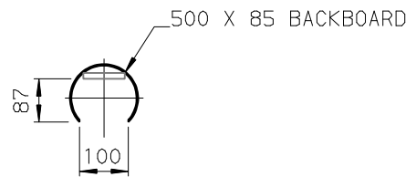
BASE COMPARTMENT. SCALE 1:10
