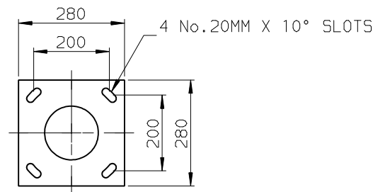
FLANGE PLATE OPTION. SCALE 1:10
